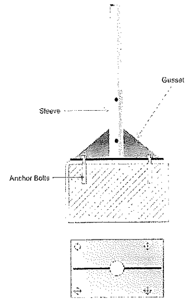
Roof Horizontal Mounted Bracket
