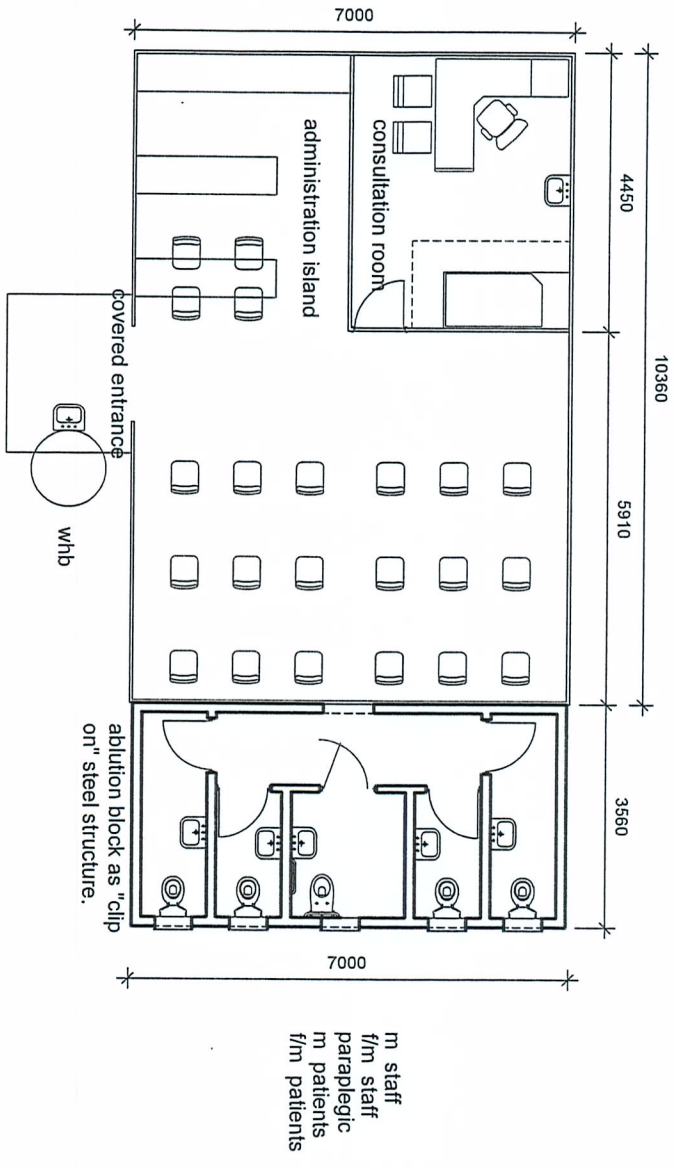
TENTED FLU CLINIC - scale 1:100
