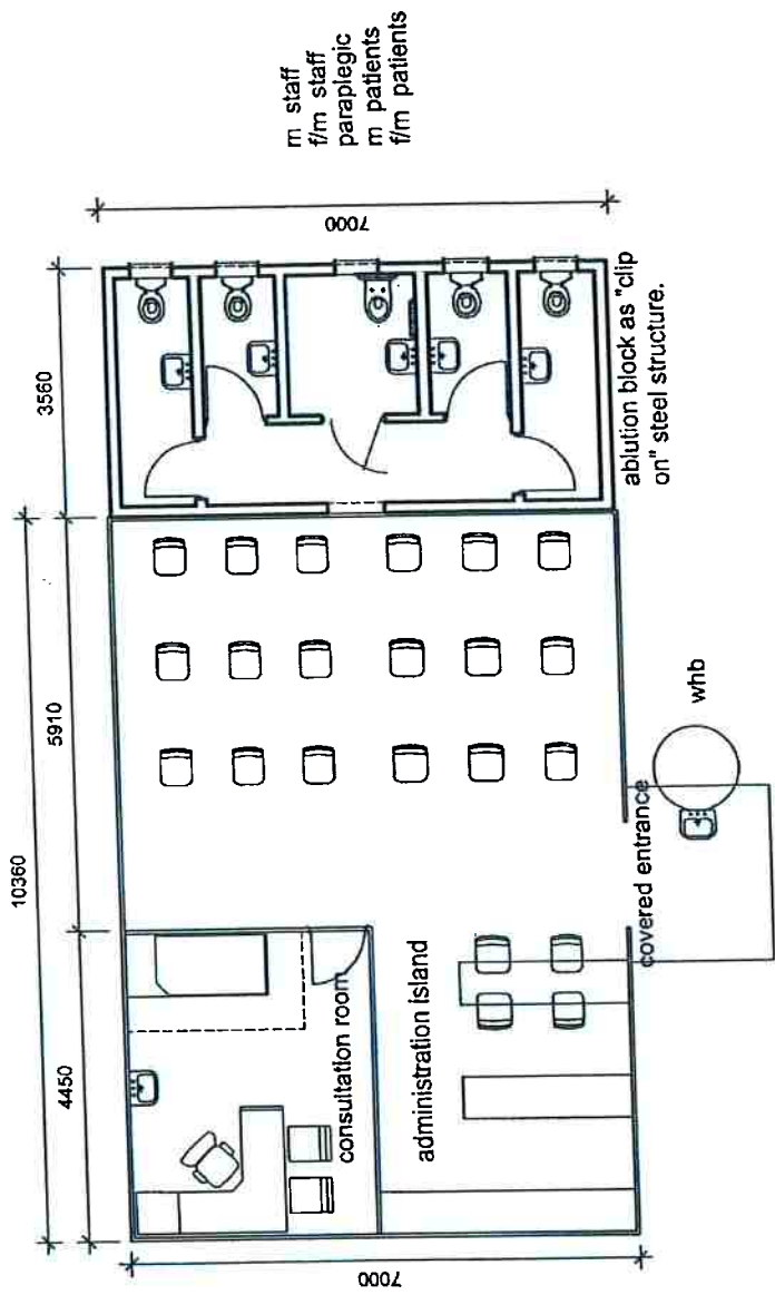
TENTED FLU CLINIC - scale 1:100
