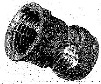
15MM COPPER TO FEMALE IRON
