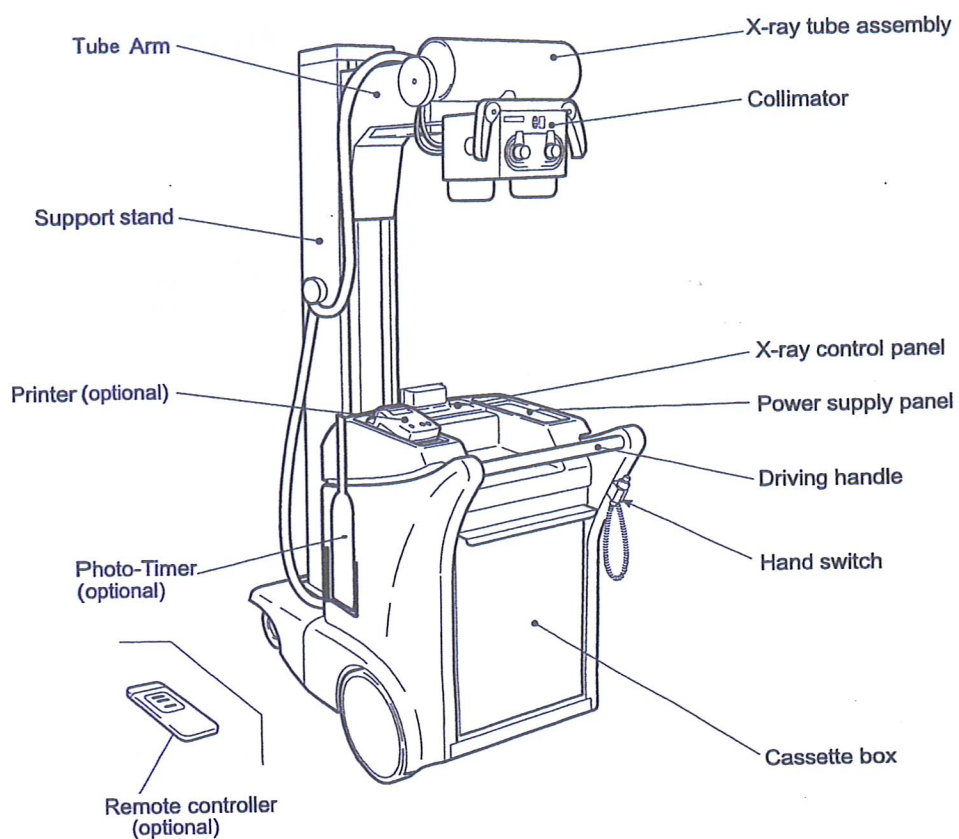
Fig. 3-1 Outside view of the system
