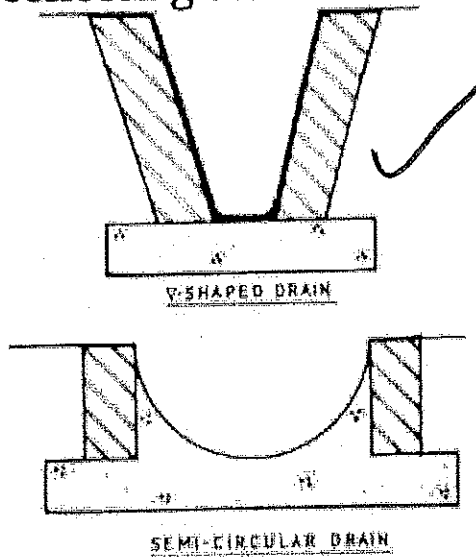
Fig. 21.4 Shapes of surface drains.
