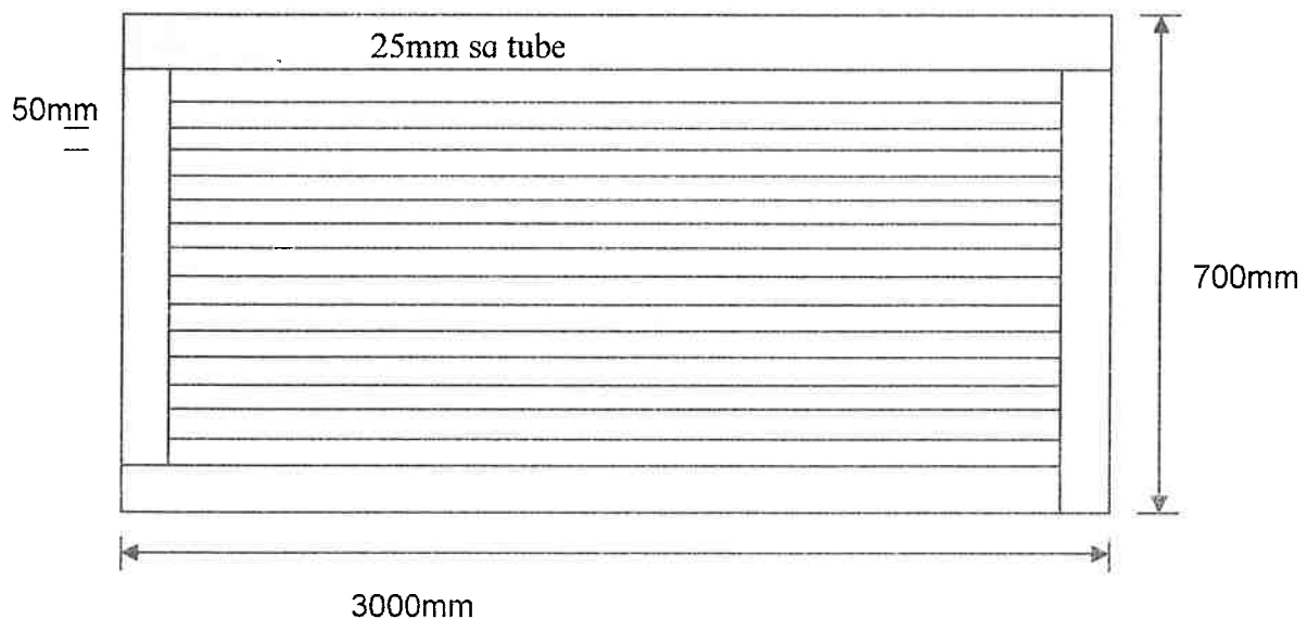
Figure 1: Top View
