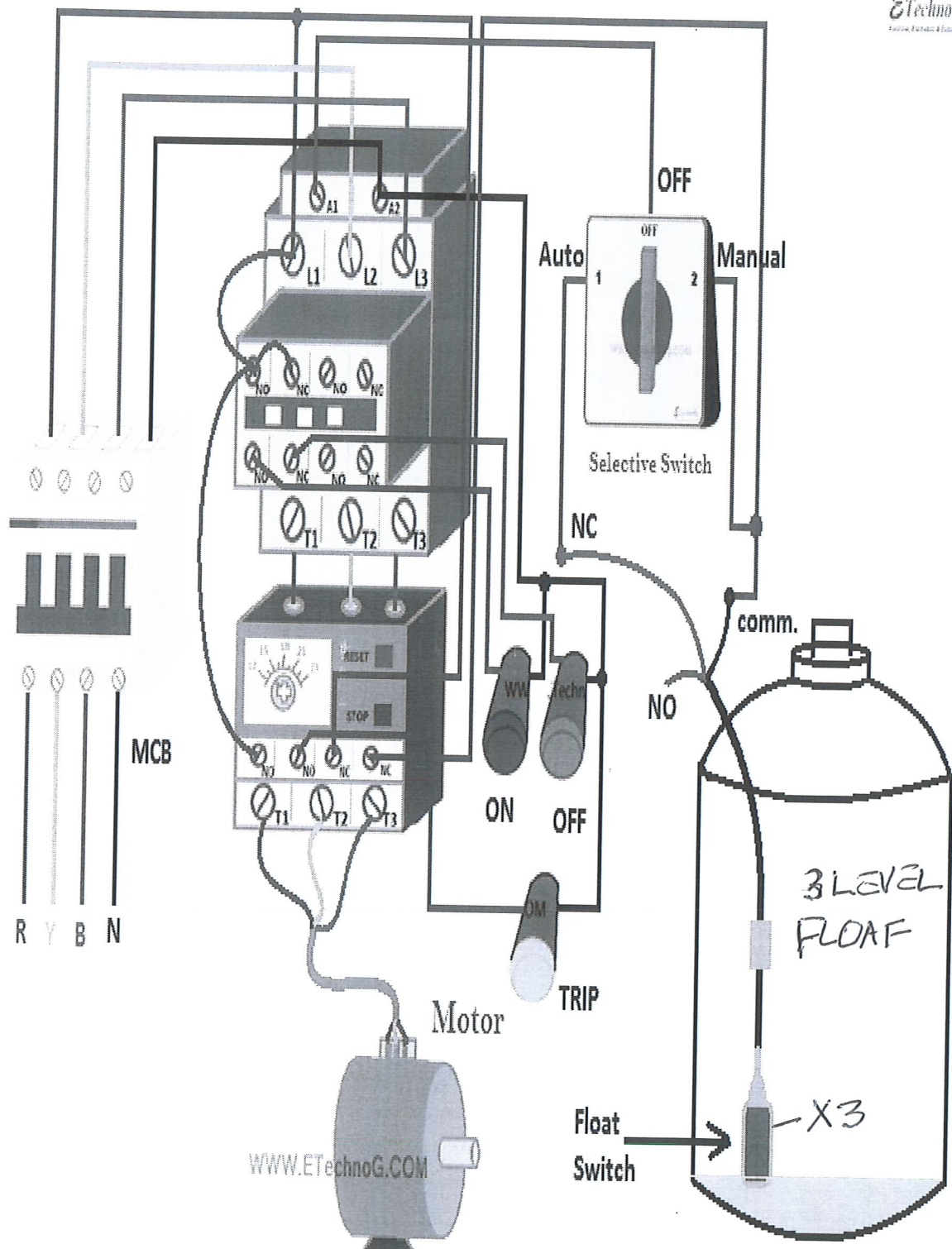
Float Switch Connection Diagram for Water Pump
