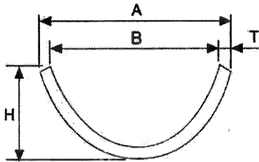
Flolok channel
