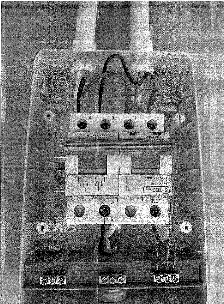
EDCO-2P-63A din rail mounted manual changeover
