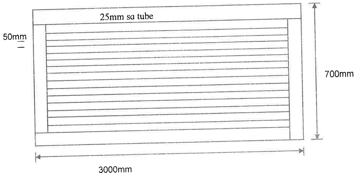
Figure 1: Top View
