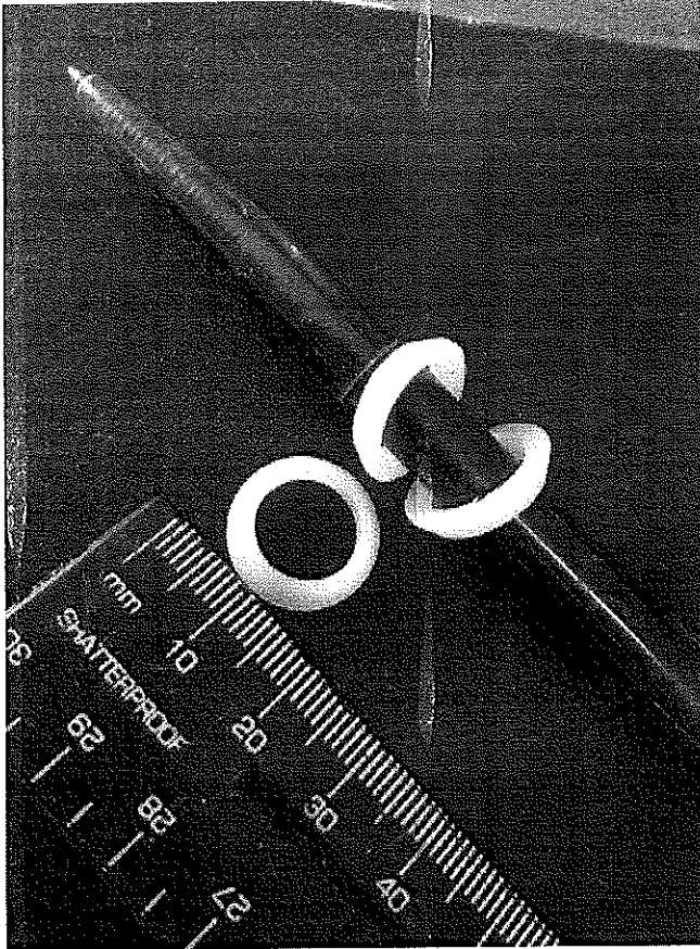
Teflon medical oxygen pigtail seal rings. Medical gas manifold by Lewthwaite engineering
