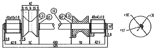
SHAFT ROLLER ASSEMBLY SCALE NTS
