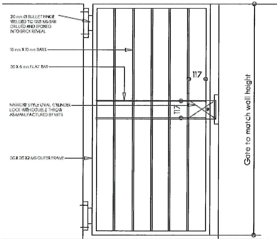
1:10 TYPICAL GATE DETAIL
