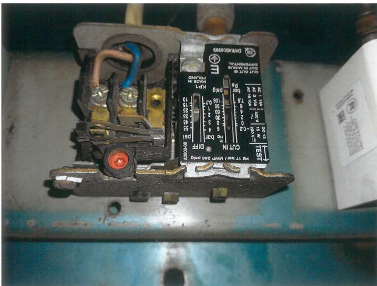
PRESSURE SWITCHES -
