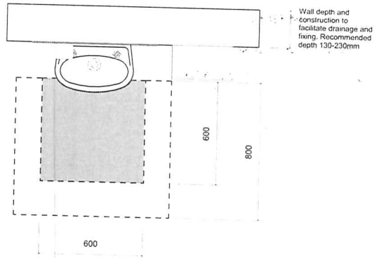
1 PLAN - NON-CLINICAL WHB 1 : 20
