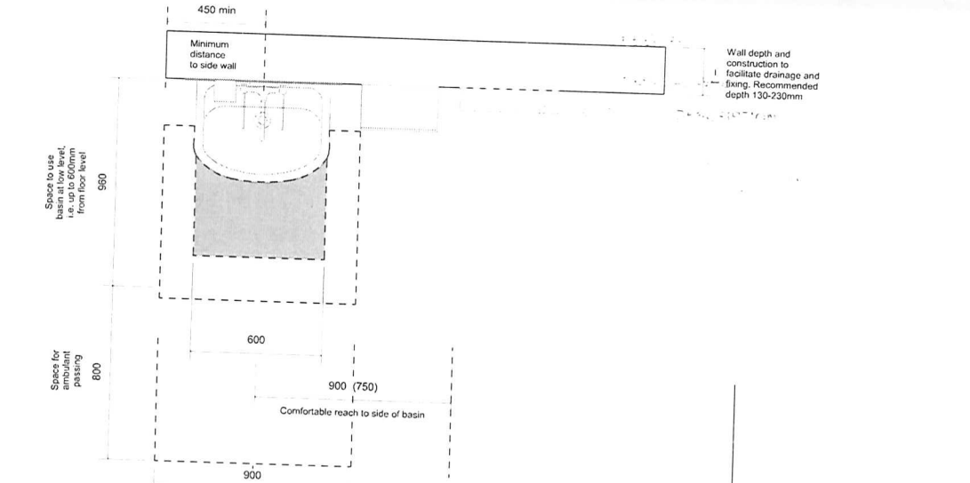
1 PLAN - CLINICAL WHB 1 : 20
