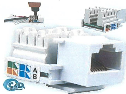
RJ45 CAT 5e wall network point jack
