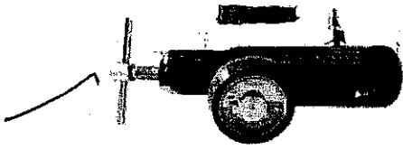
Regulator, pin index, dial click stop constant flow, pressure gauge to register cylinder pressure, oxygen, outer body aluminum, inner liner brass
