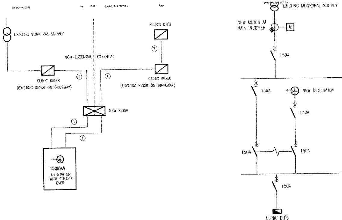
Figure 2: Generator Schematic
