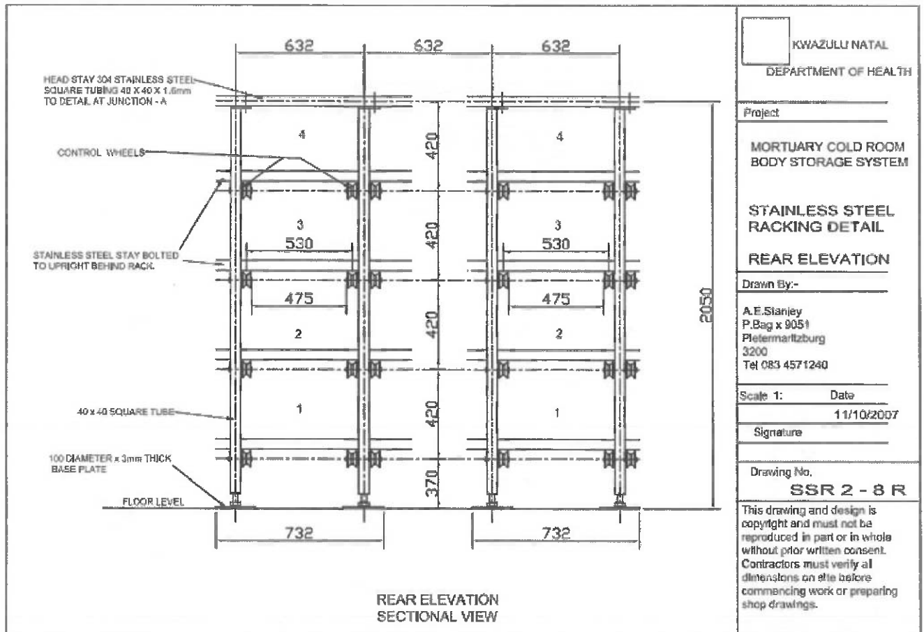
FIGURE 3: REAR ELEVATION SECTIONAL VIEW (ABOVE)
