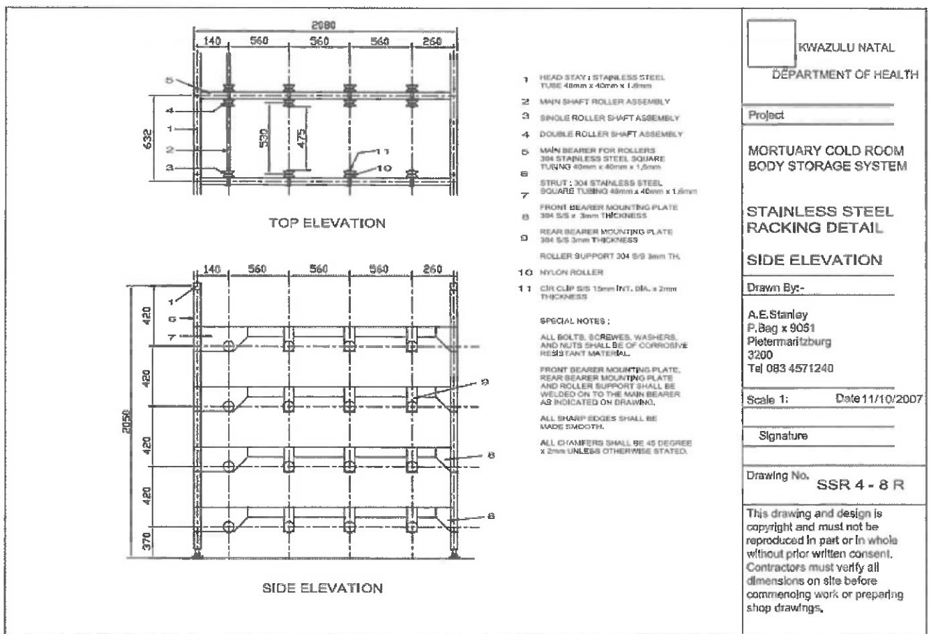
FIGURE 4: SIDE ELEVATION (ABOVE)
