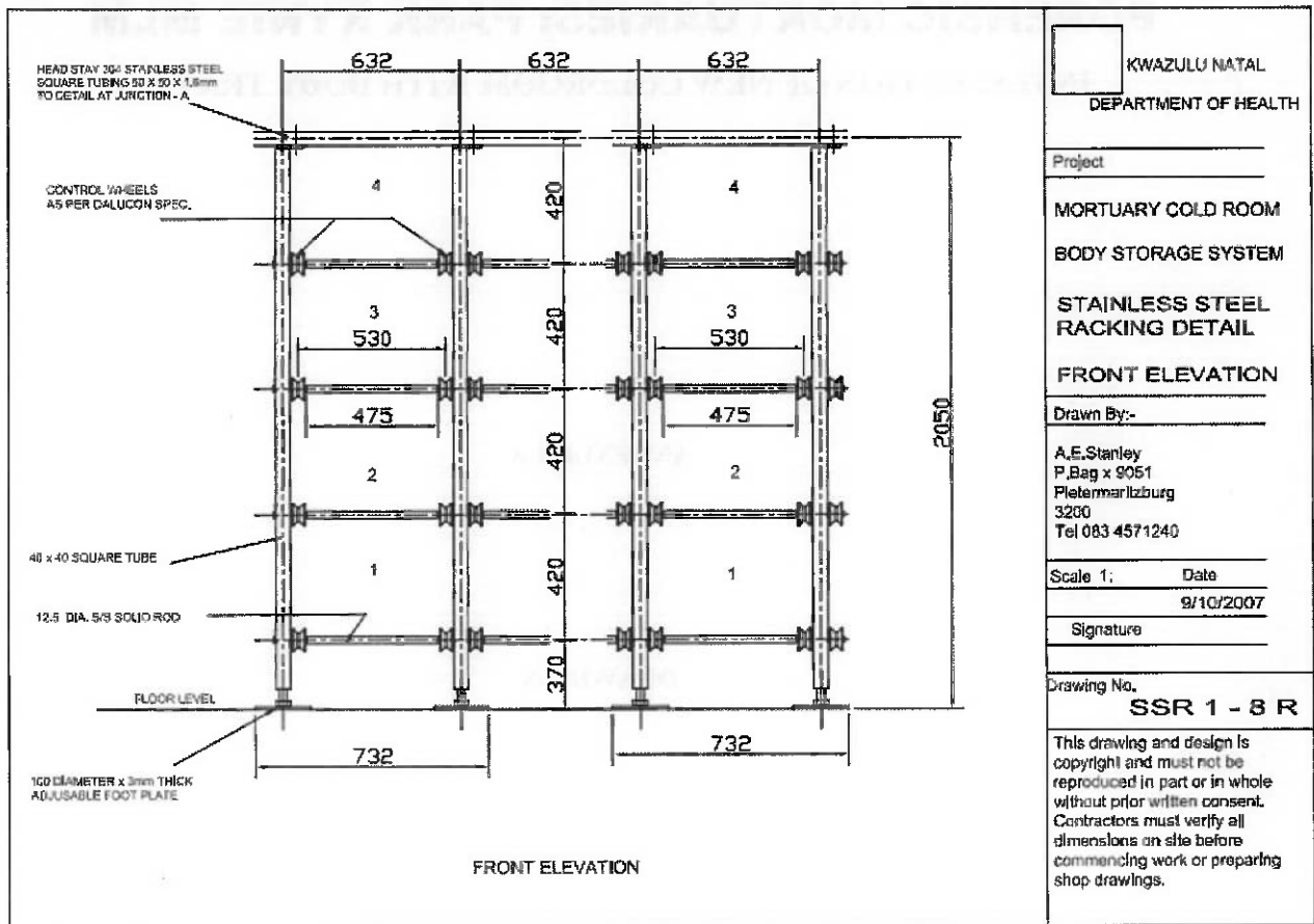
FIGURE 1 : FRONT ELEVATION (ABOVE)
