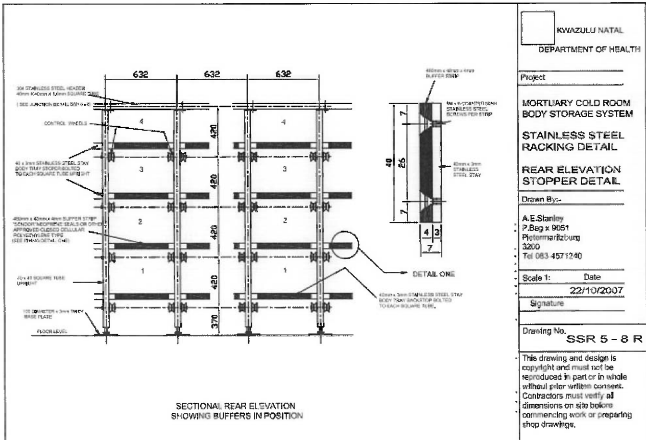
FIGURE 2: REAR ELEVATION STOPPER DETAIL (ABOVE)
