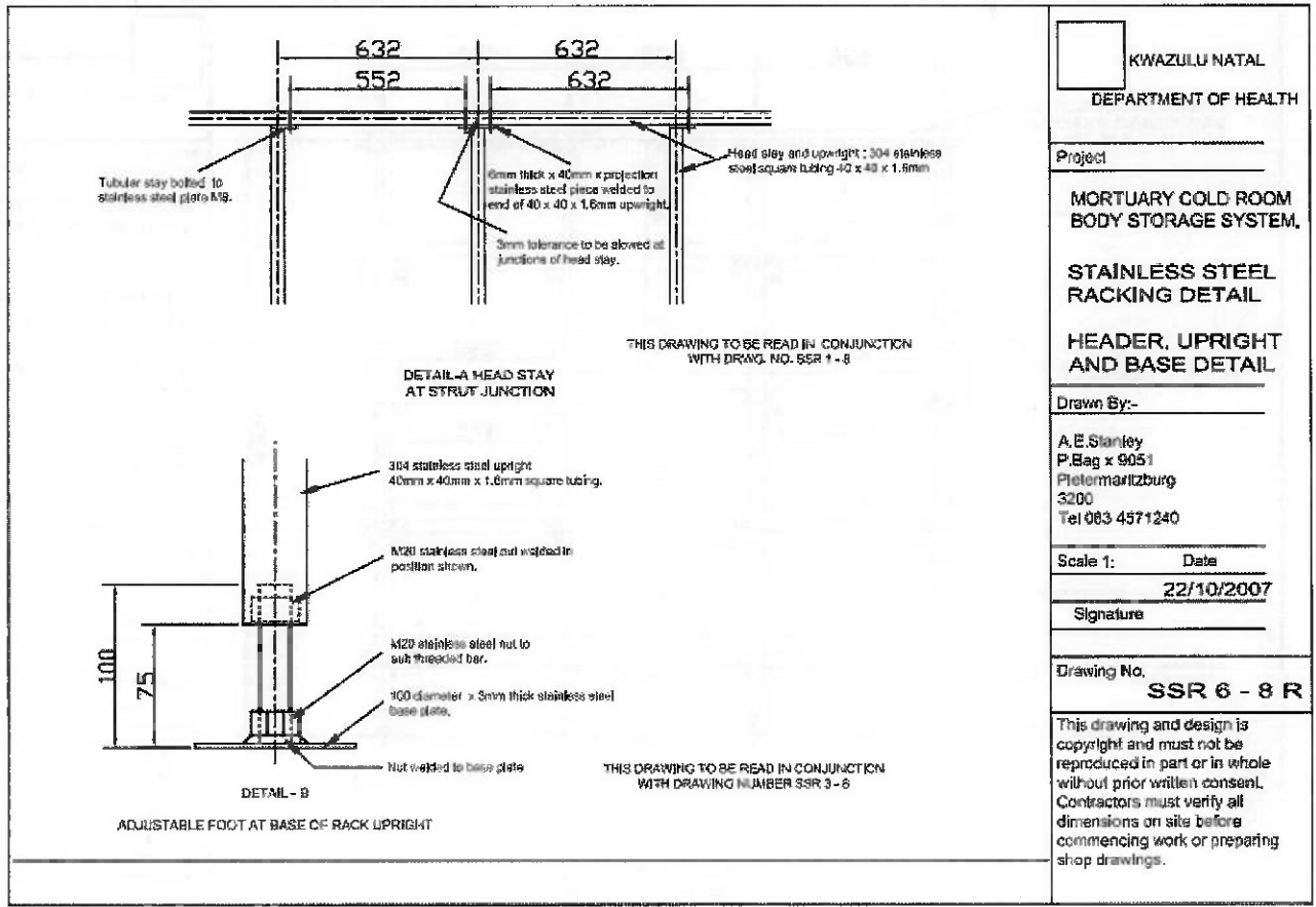
FIGURE 5: HEADER UPRIGHT AND BASE DETAIL
